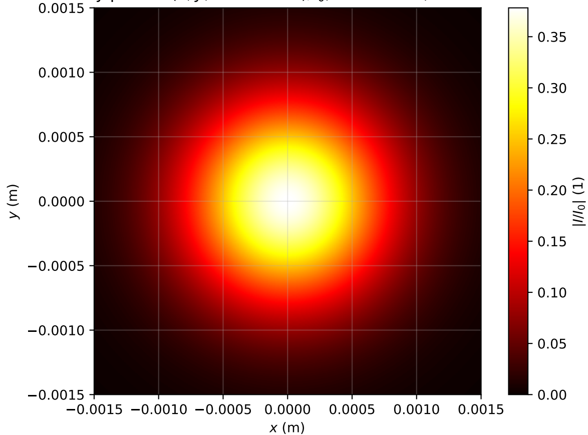
Intensity profile I(x, y, z = 3.264m)/I_0 , P_{in}=0.3P_{cr} , artificial time
